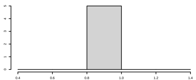
Density of rho.eps2[1,1]
