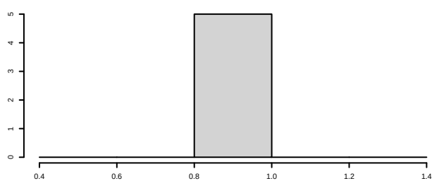
Density of rho.eps2[2,2]
